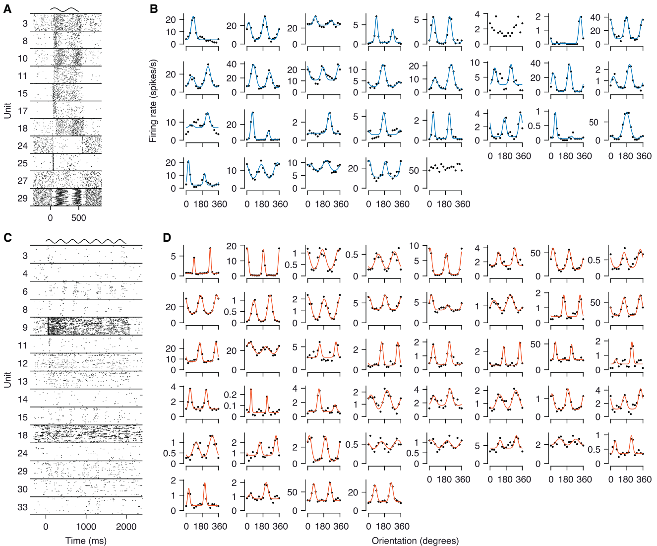
Figure 1. Recordings of Population Activity in V1
